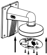
Figure 1-15 Secure the Adapter
