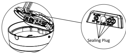
Figure 1-9 Route the Cables
