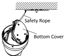
Figure 1-8 Hook the Camera to the Adapter
