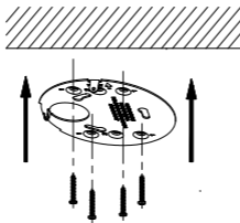
Figure 1-7 Secure the Adapter to the Ceiling
