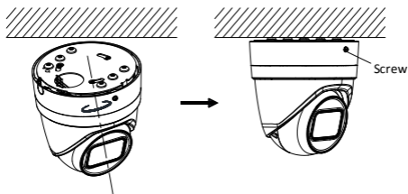
Figure 1-10 Secure the Camera
