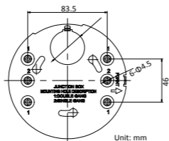
Figure 1-6 Drill Holes in the Ceiling
